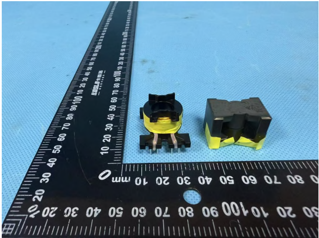
Figure 7.: Detail view of transformer TS1
