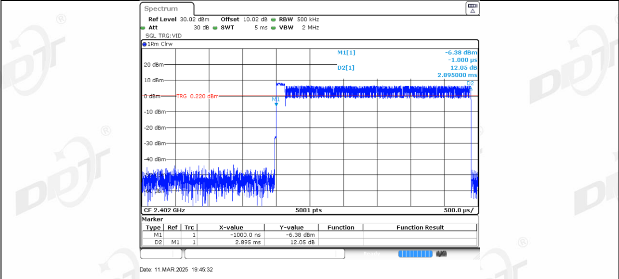
2DH5_Ant1_Hop_2402
