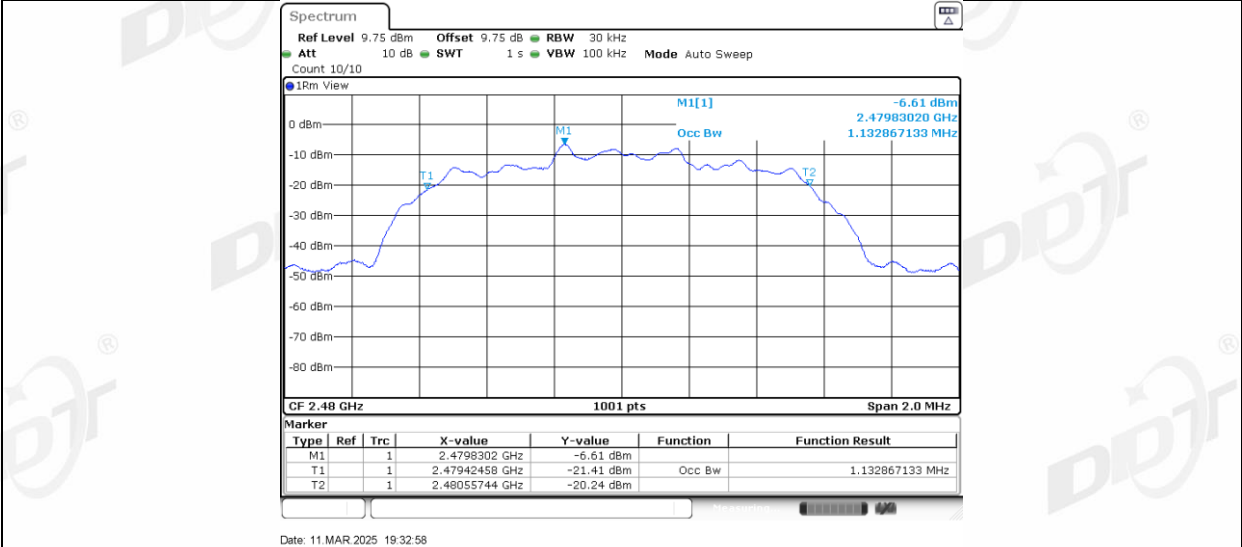
2DH5_Ant1_2402
