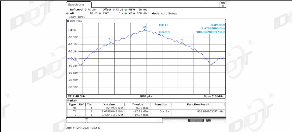
2DH1_Ant1_2402
