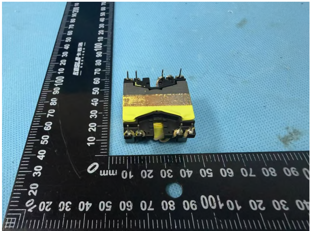
Figure 5.: Detail view of transformer TS1
