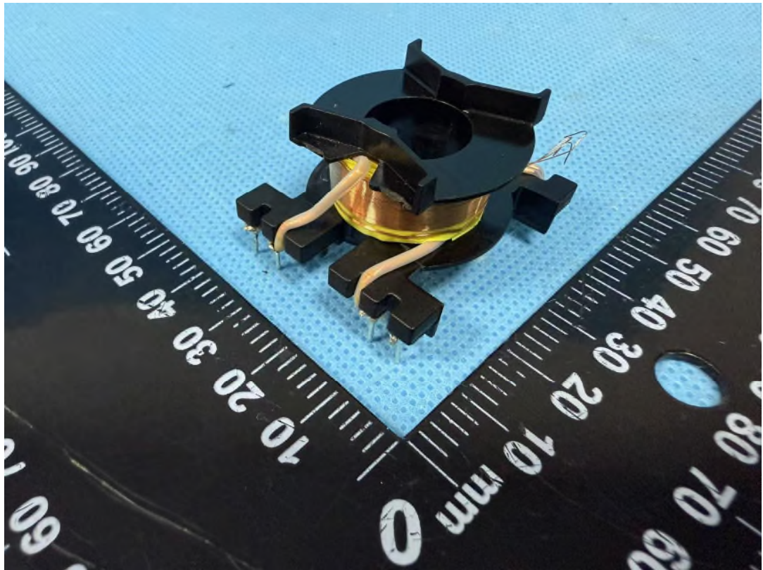
Figure 9.: Detail view of transformer TS1
