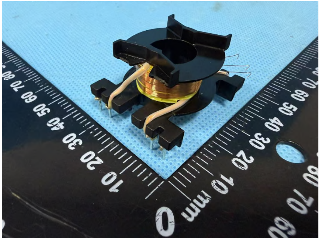
Figure 11.: Detail view of transformer TS1
