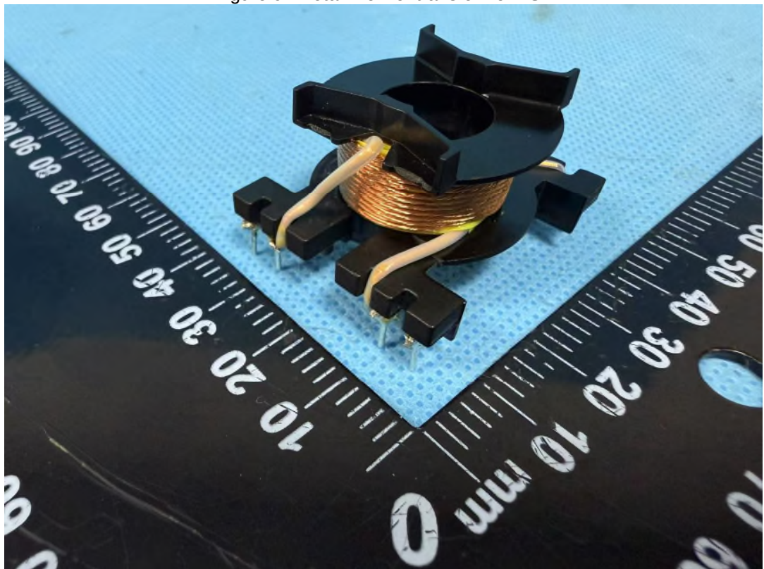
Figure 10.: Detail view of transformer TS1
