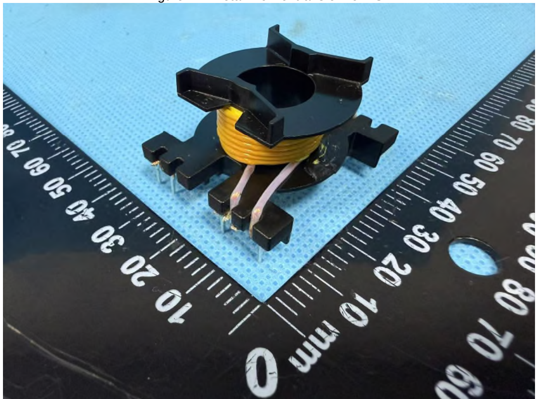
Figure 12.: Detail view of transformer TS1
