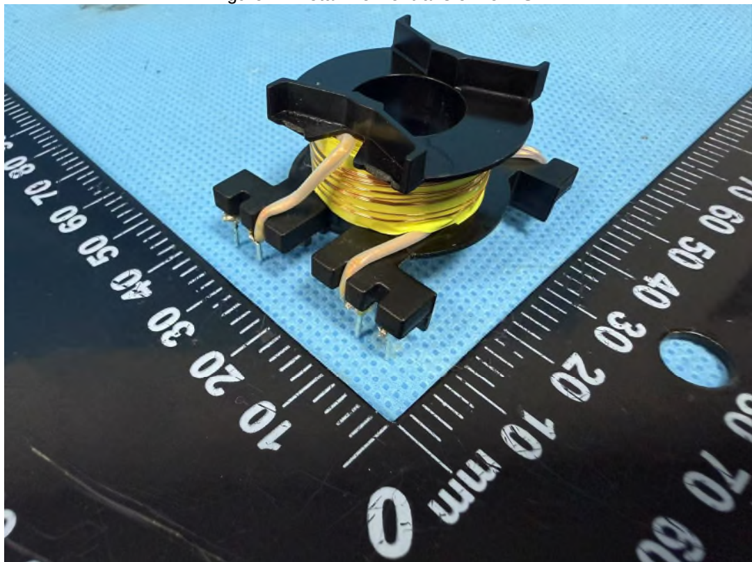
Figure 8.: Detail view of transformer TS1
