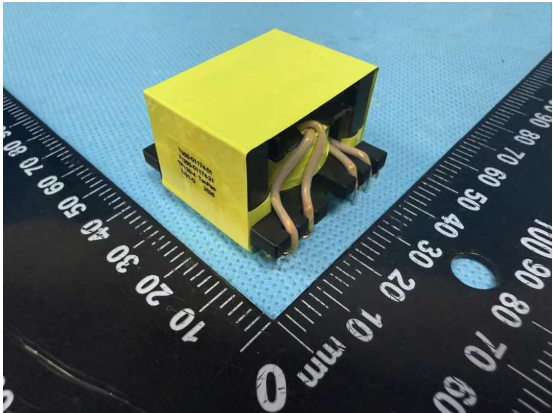
Figure 3.: Detail view of transformer TS1
