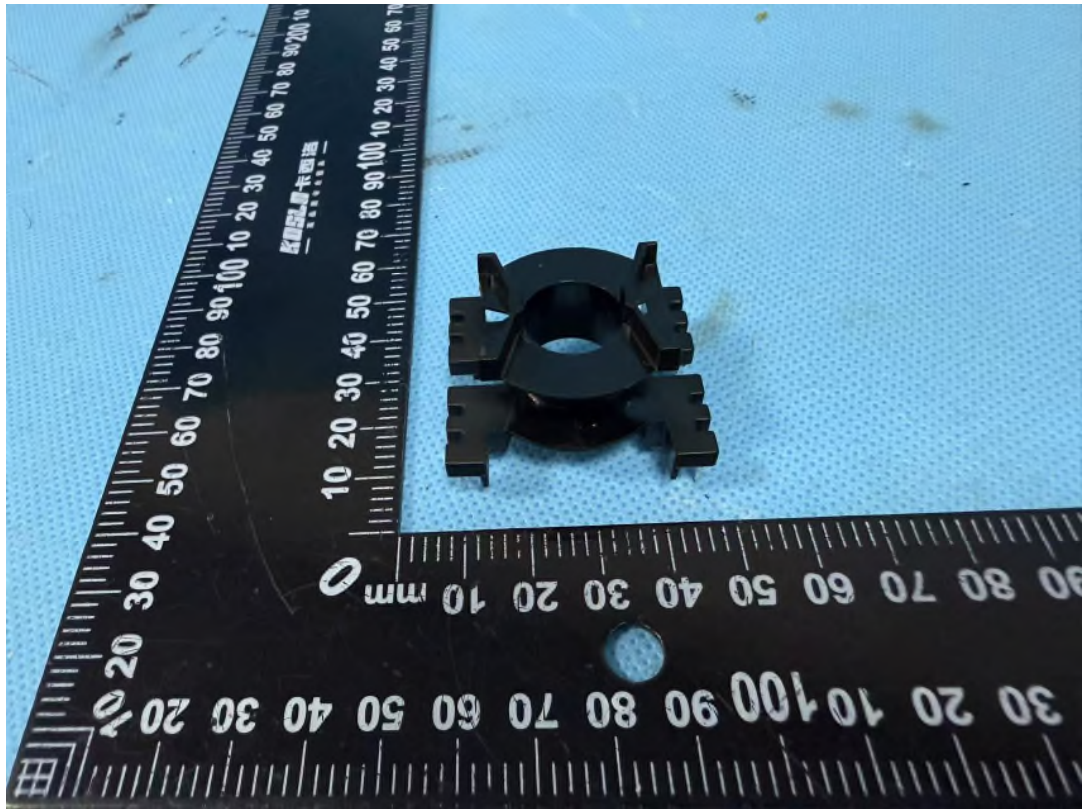
Figure 13.: Detail view of transformer TS1
